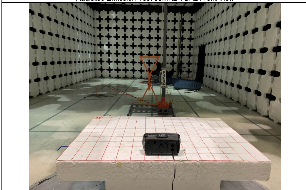
Radiated Emission Test 30MHz-1GHz Rear View
