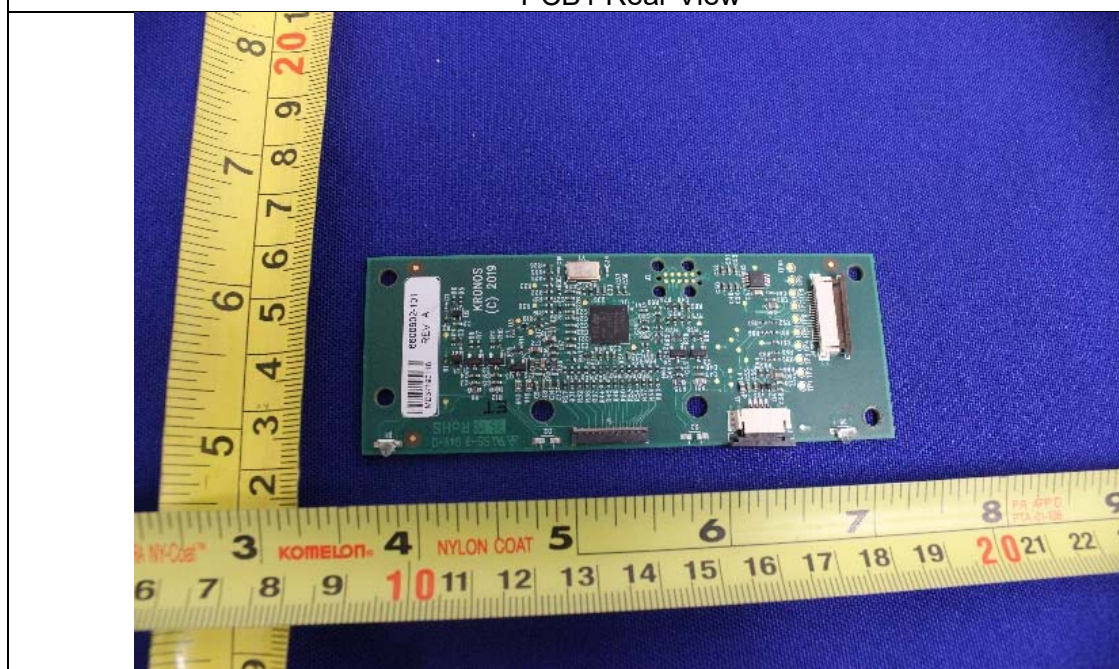
PCB2 Front View
