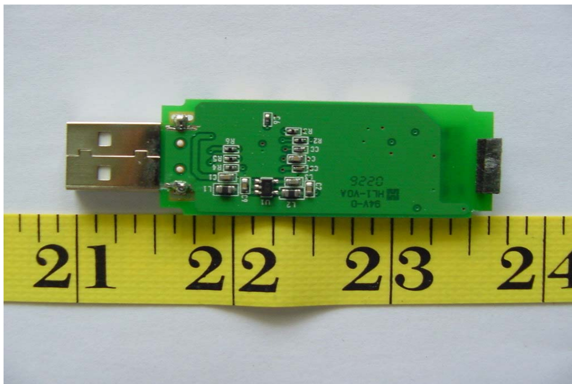
6. Solder View of Main PCB
