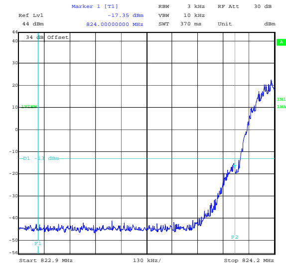
Title: 49304JD07 FCC PART 22 Comment A: RADIATED BAND EDGE BOTTOM CHANNEL GSM850 Date: 13.DEC.2007 15:12:47
