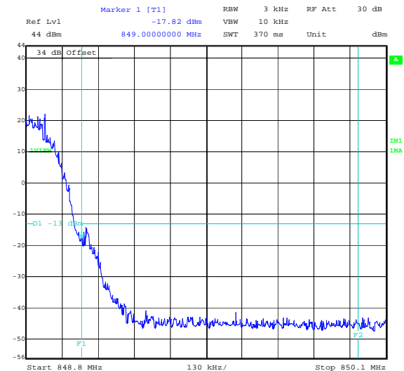
Title: 49304JD07 FCC PART 22 Comment A: RADIATED BAND EDGE TOP CHANNEL GSM850 Date: 13.DEC.2007 15:17:02
