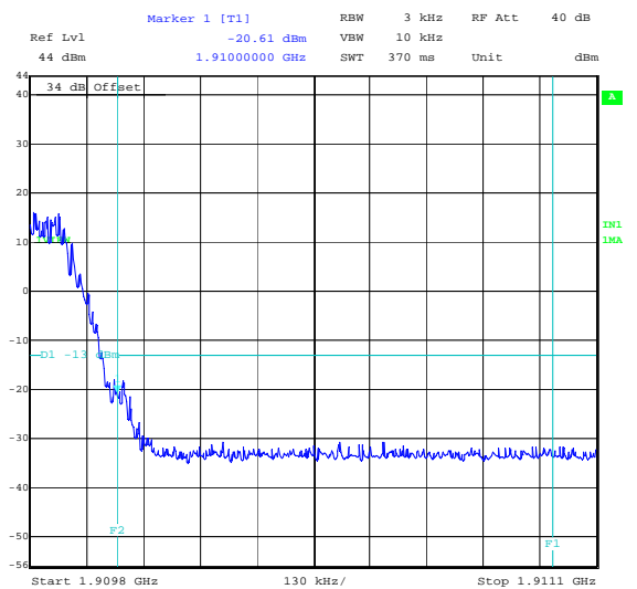
Title: 49304JD07 FCC PART 24 Comment A: RADIATED BAND EDGE TOP CHANNEL EGPRS1900 Date: 13.DEC.2007 12:32:11
