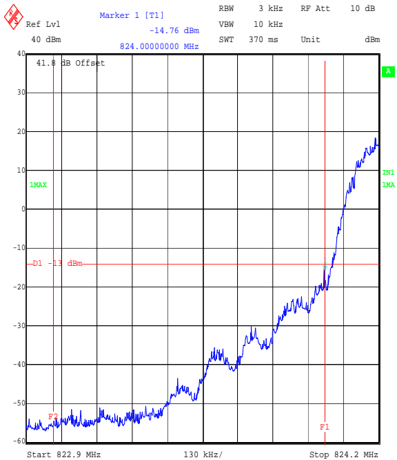
Title: Flextronic EUT: G32a FCC Part 22. Radiated Band Edge Comment A: 48122JD03 Operating in GSM 850, Bottom Channel, GPRS Mode. Date: 10.JUL.2006 12:31:39
