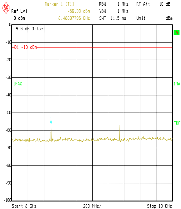
Title: Flextronic EUT: 6120, FCC P22 Radiated Emissions Comment A: 48122JD03 Tx Mode, Top Channel, GSM 850 Date: 04.MAY 2006 18:43:34
