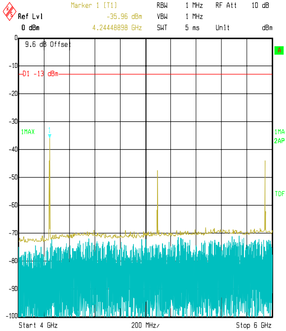
Title: Flextronic EUT: 6120, FCC P22 Radiated Emissions Comment A: 48122JD03 Tx Mode, Top Channel, GSM 850 Date: 04.MAY 2006 17:43:56
