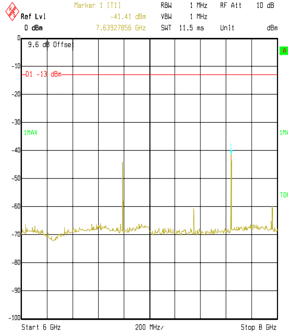
Title: Flextronic EUT: 6120, FCC P22 Radiated Emissions Comment A: 48122JD03 Tx Mode, Top Channel, GSM 850 Date: 04.MAY 2006 18:27:59
