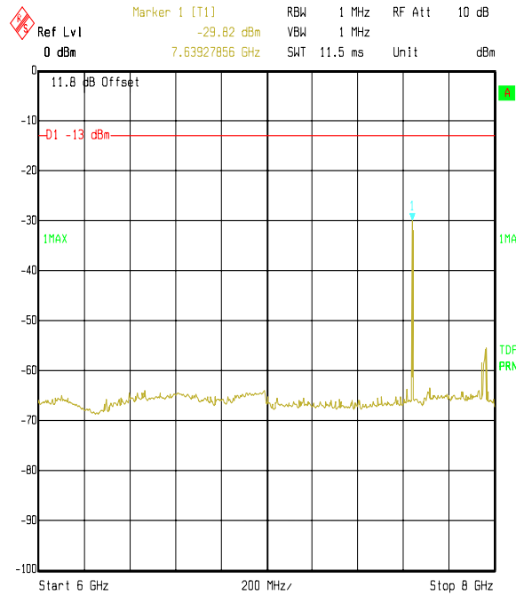
Title: Flextronic EUT: 6120, FCC P24 Radiated Emissions Comment A: 48122JD03 Tx Mode, Top Channel, GSM 1900 Date: 04.MAY 2006 18:30:25
