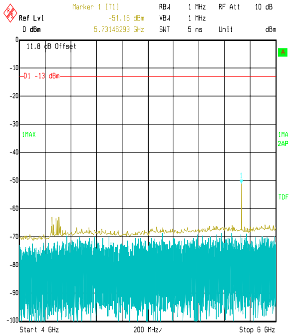
Title: Flextronic EUT: 6120, FCC P24 Radiated Emissions Comment A: 48122JD03 Tx Mode, Top Channel, GSM 1900 Date: 04.MAY 2006 17:39:43
