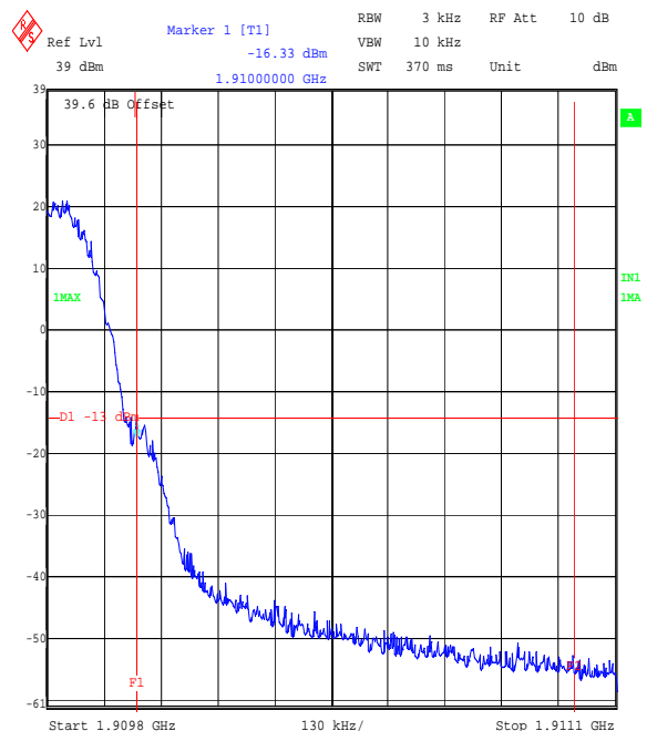
Title: Flextronic EUT: G32a FCC Part 24. Radiated Band Edge Comment A: 48122JD03 Operating in PCS 1900, Top Channel, EDGE Mode. Date: 10.JUL.2006 12:02:35
