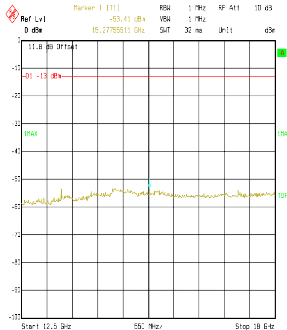
Title: Flextronic EUT: 6120, FCC P24 Radiated Emissions Comment A: 48122JD03 Tx Mode, Top Channel, GSM 1900 Date: 04.MAY 2006 18:53:07
