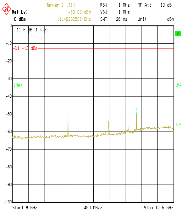
Title: Flextronic EUT: 6120, FCC P24 Radiated Emissions Comment A: 48122JD03 Tx Mode, Top Channel, GSM 1900 Date: 04.MAY 2006 18:46:25
