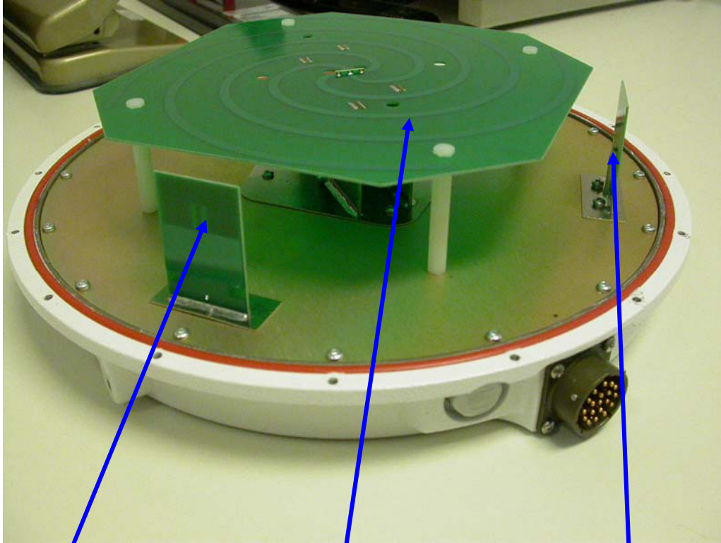
Satellite Antenna
