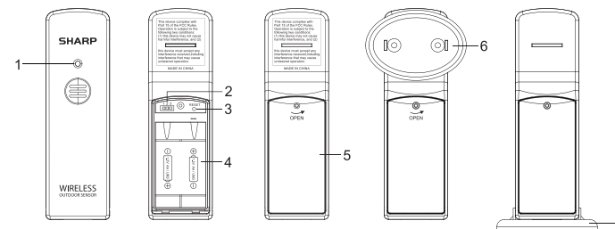
Remote Transmitter
