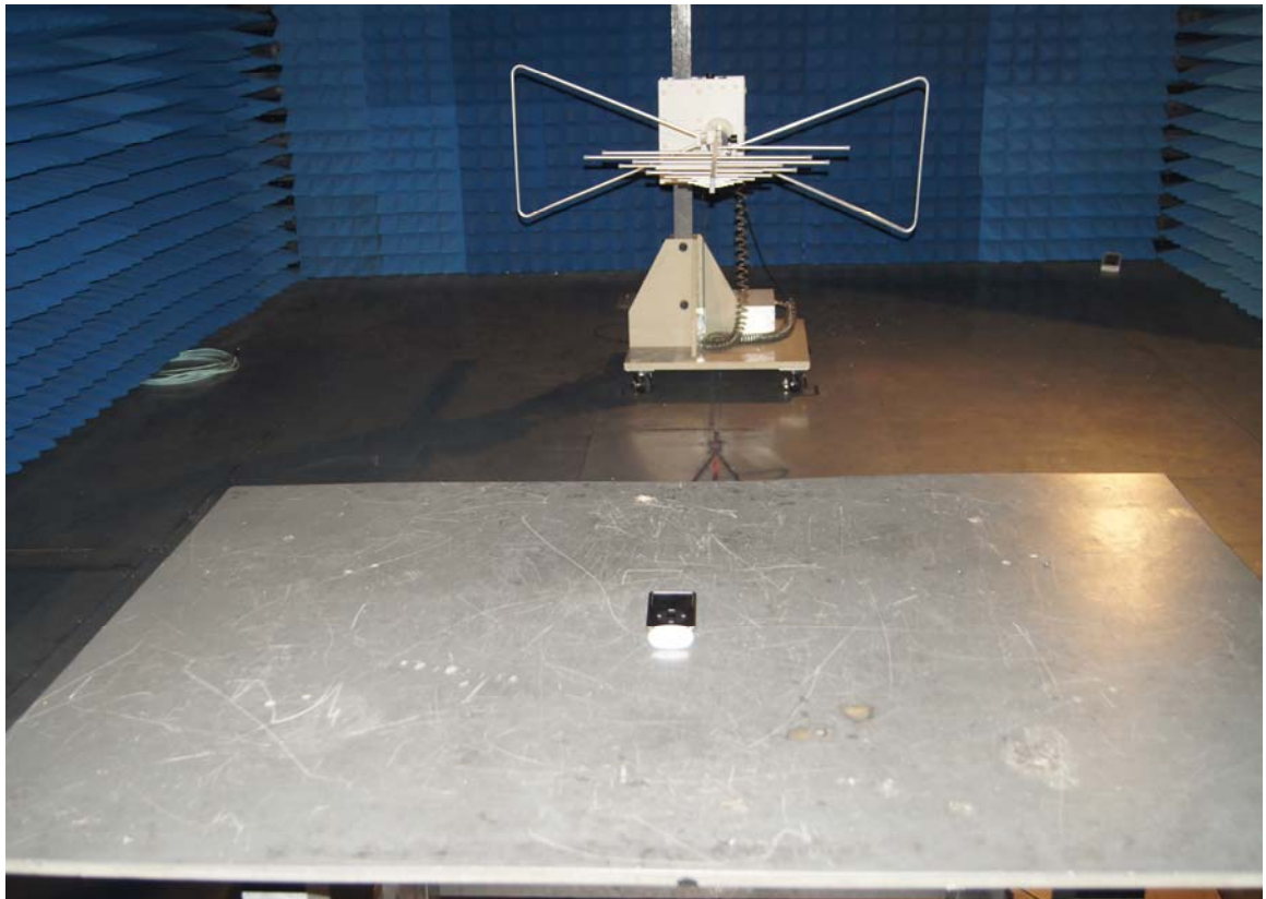
Radiated emissions test 30MHz- 1GHz
