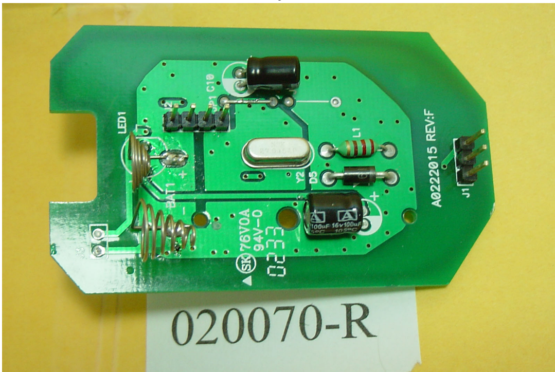
Internal of EUT – 1
