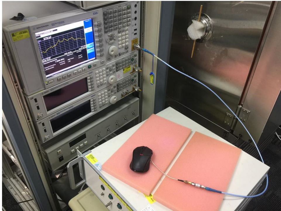
Photograph 4: Set-up for Conducted measurement
