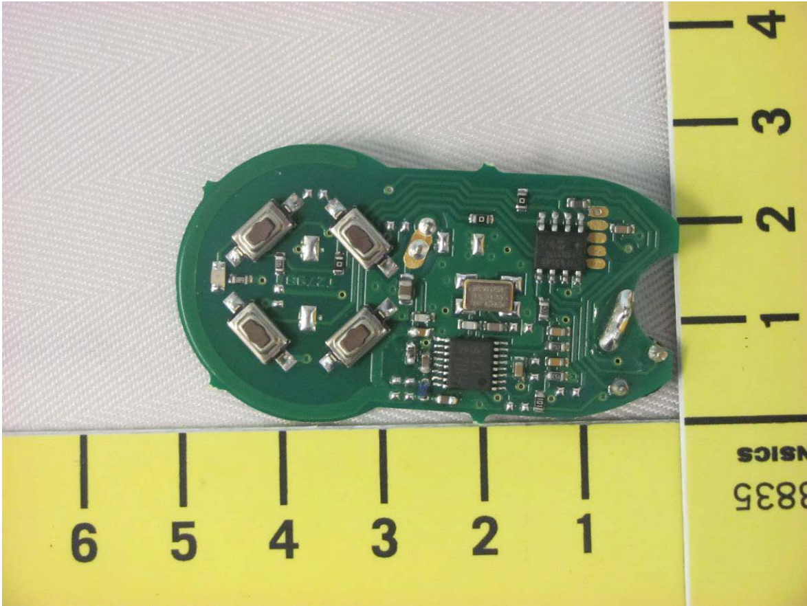
Illustration 1: EUT internal view - front
