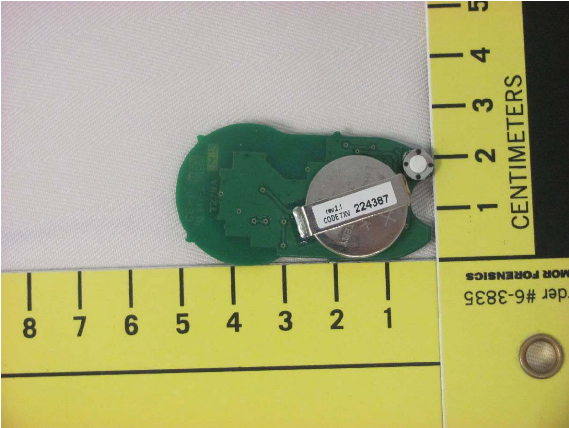
Illustration 3: EUT internal view – rear with battery
