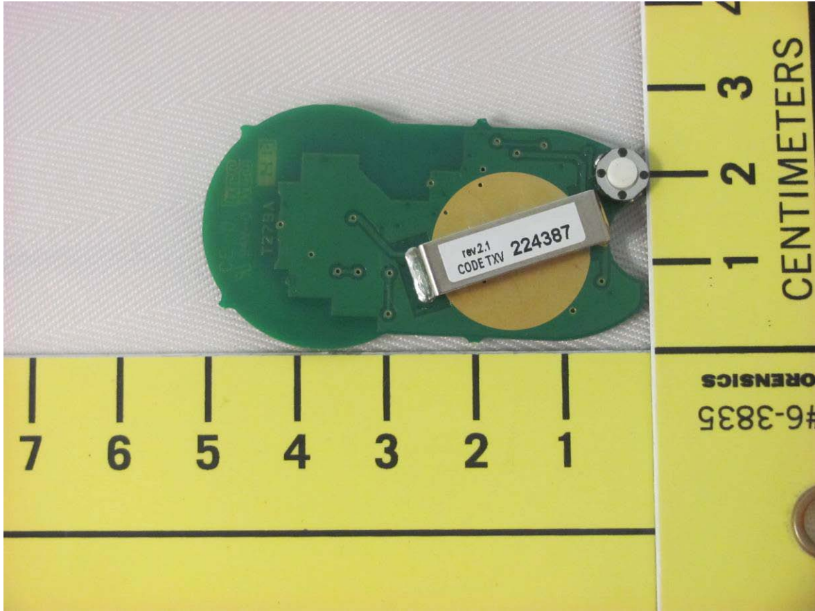
Illustration 2: EUT internal view - rear
