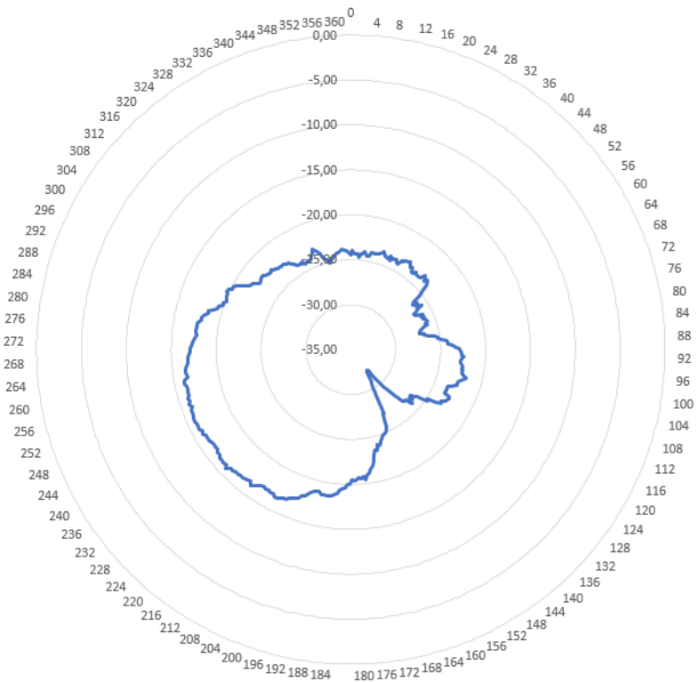
916 MHz Horizontal antenna
