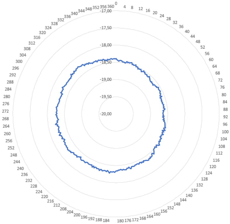
433 MHz Vertical antenna
