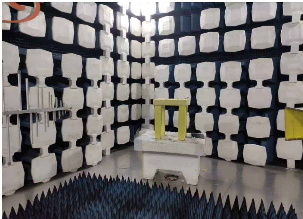
Description: Test Setup(model: EMC3290-S)
