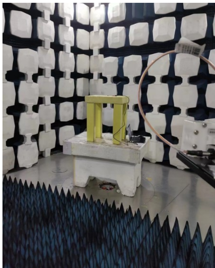
Description: Test Setup(model: EMC3290-S)
