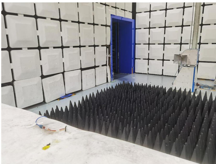
Description: Radiated Emission Test Setup for 1GHz ~ 18GHz (Mode1)
