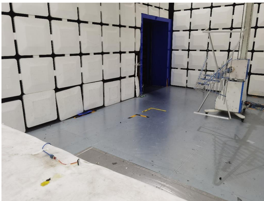
Description: Radiated Emission Test Setup for 30MHz ~ 1GHz (Mode1)
