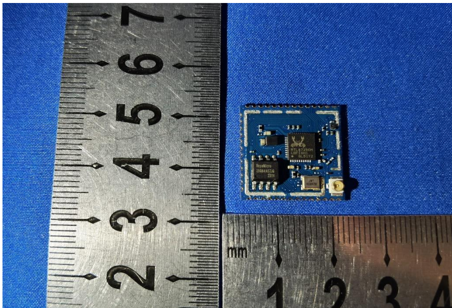
Photo 3: Internal View for PCB
