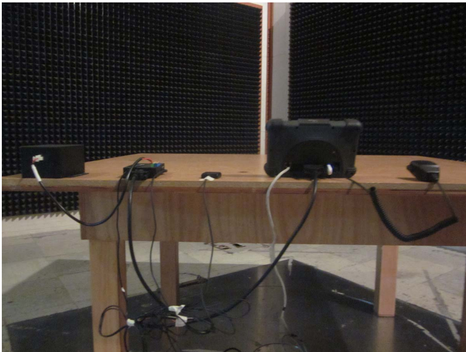
EMC_SMT-500P_Test Rear Photo (Detail View)
