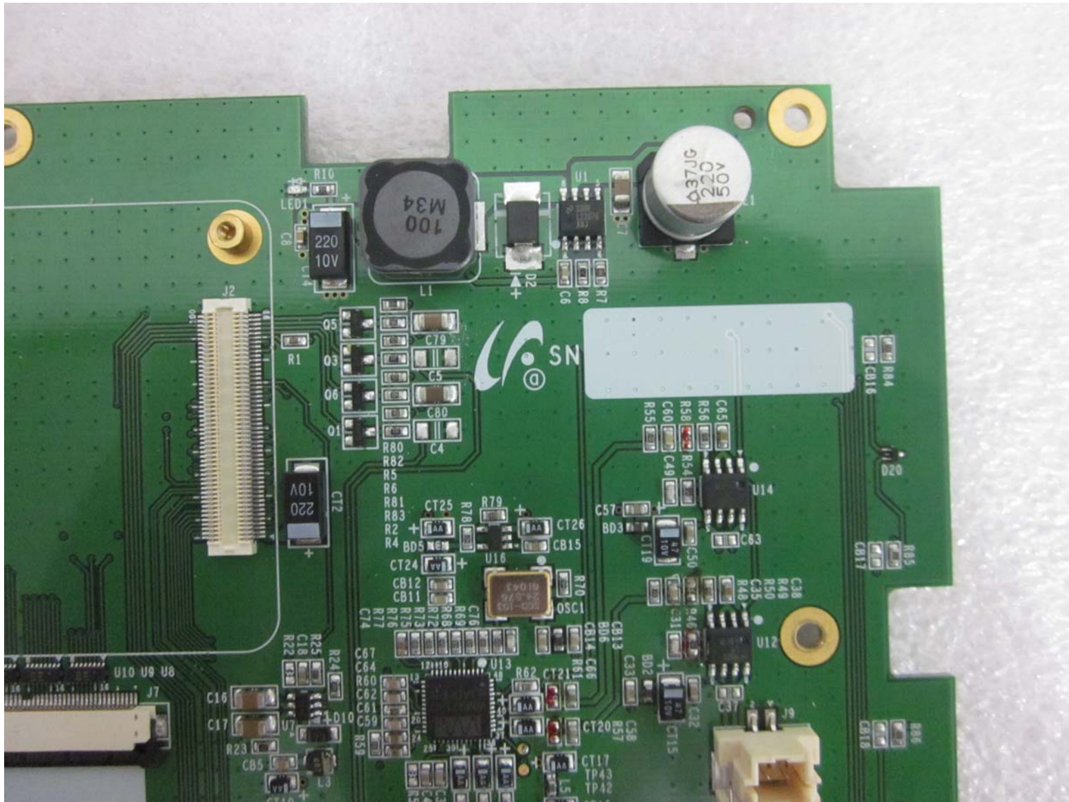
SMT-500P_Main Board Front-2
