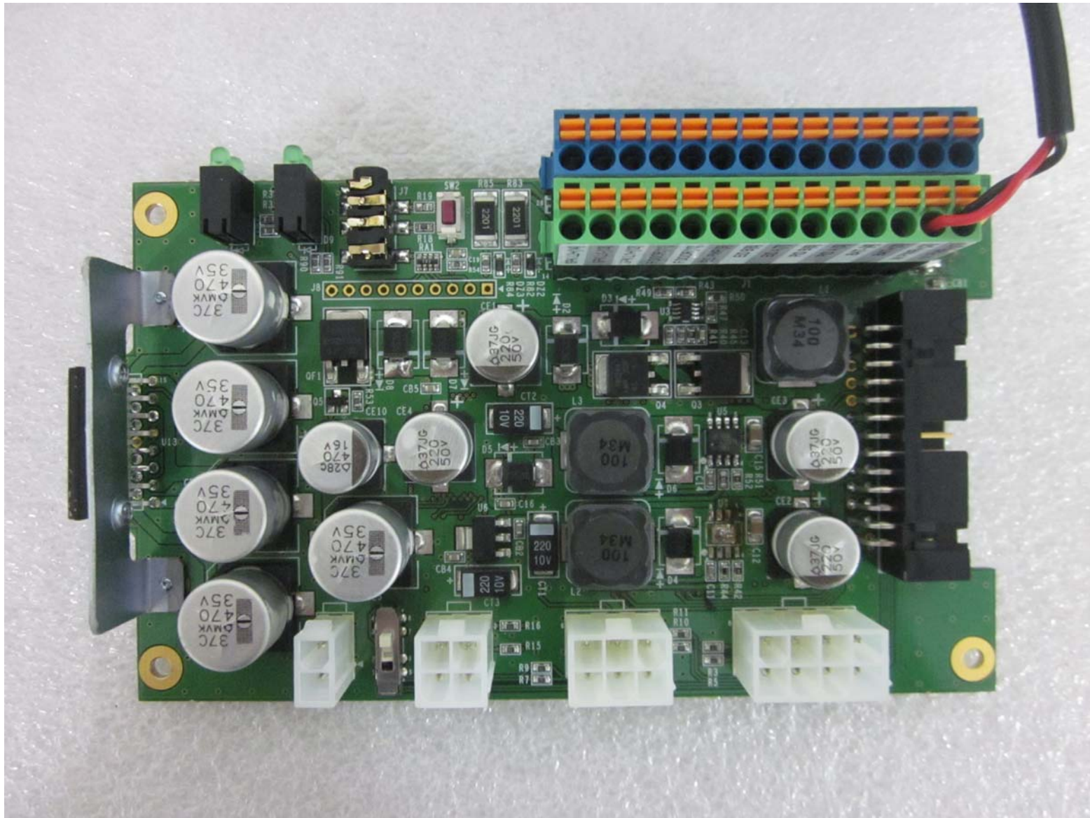
SMT-500P_Breakout Box_Main Board Front
