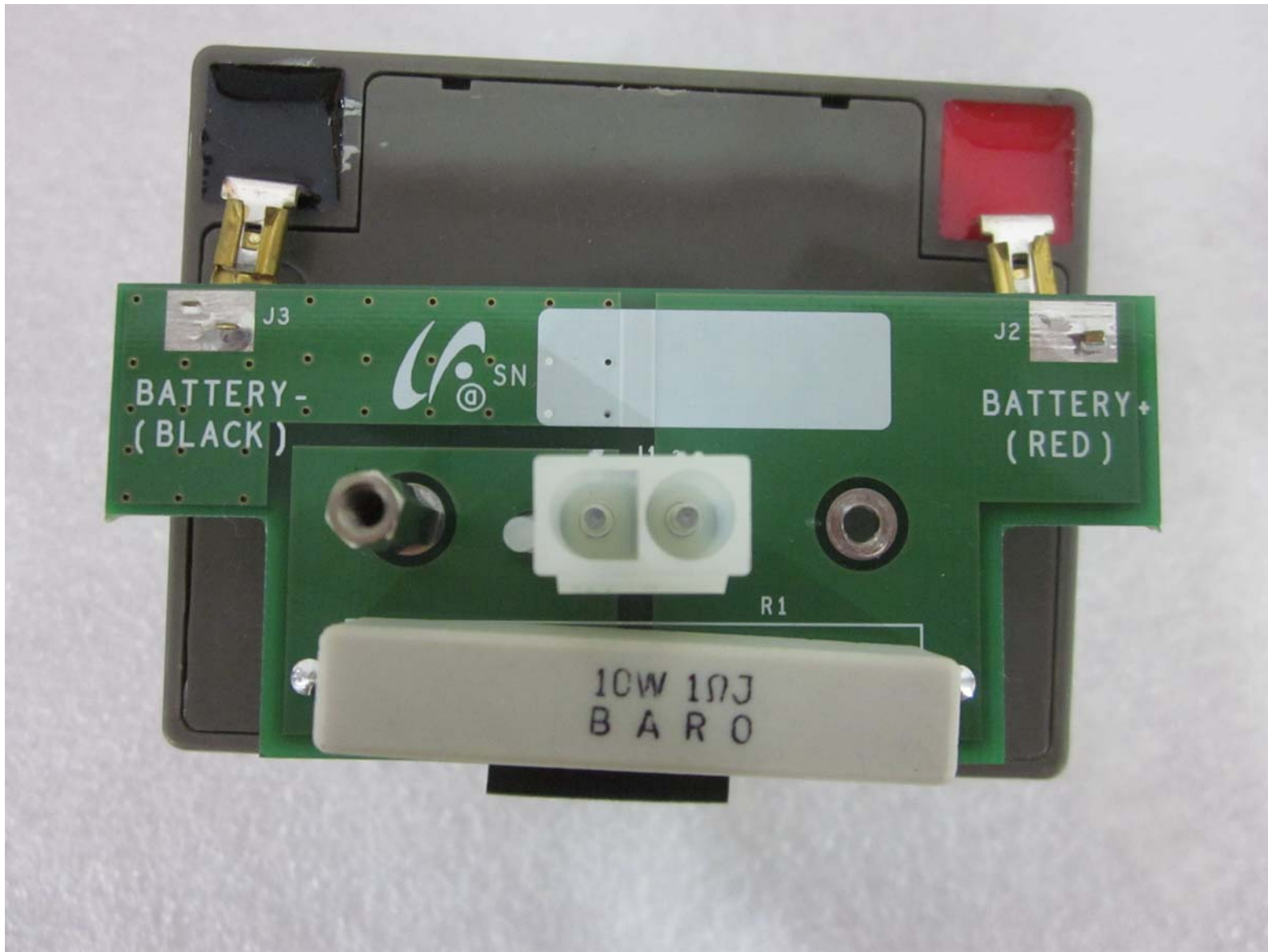
SMT-500P_Battery Pack_Main Board Front
