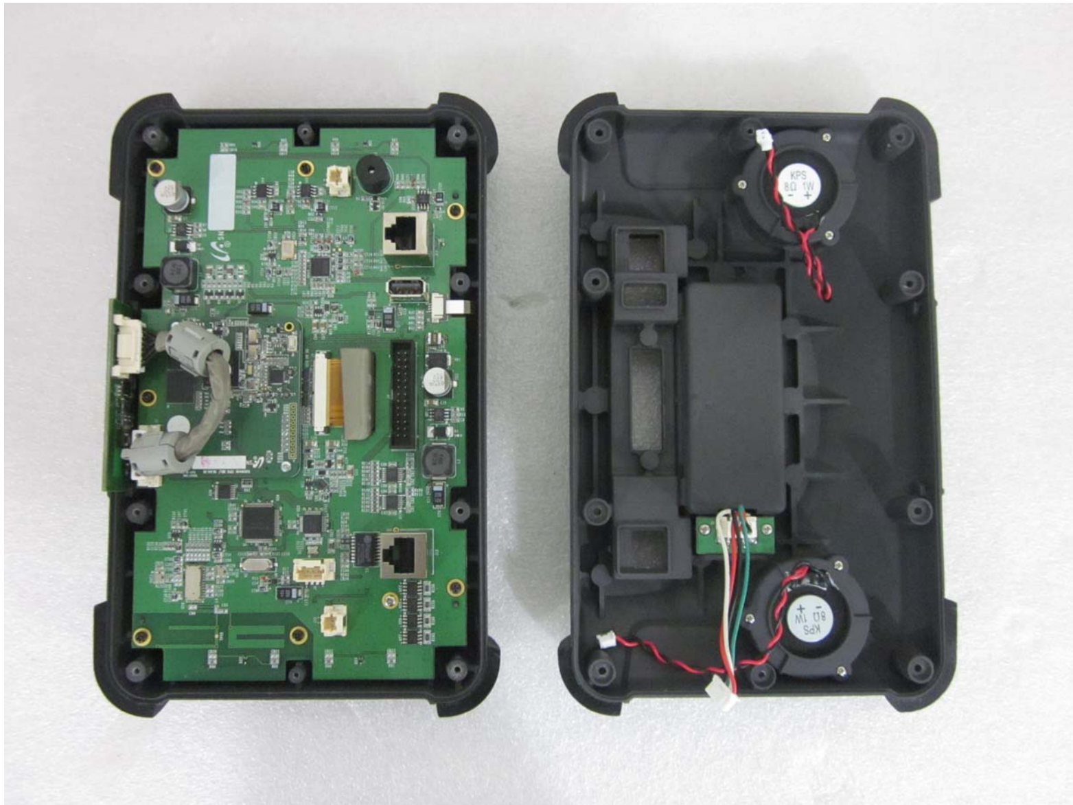
SMT-500P_inner View
