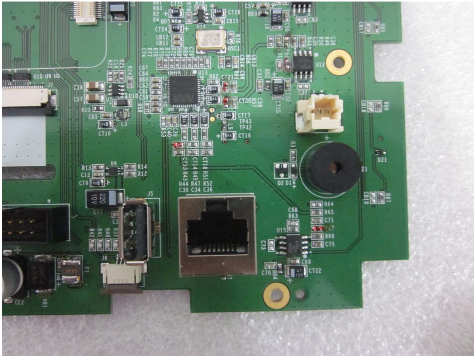
SMT-500P_Main Board Front-3
