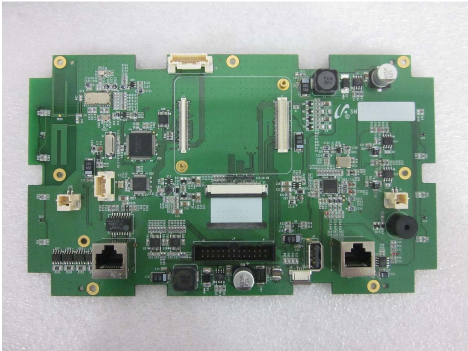
SMT-500P_Main Board Front
