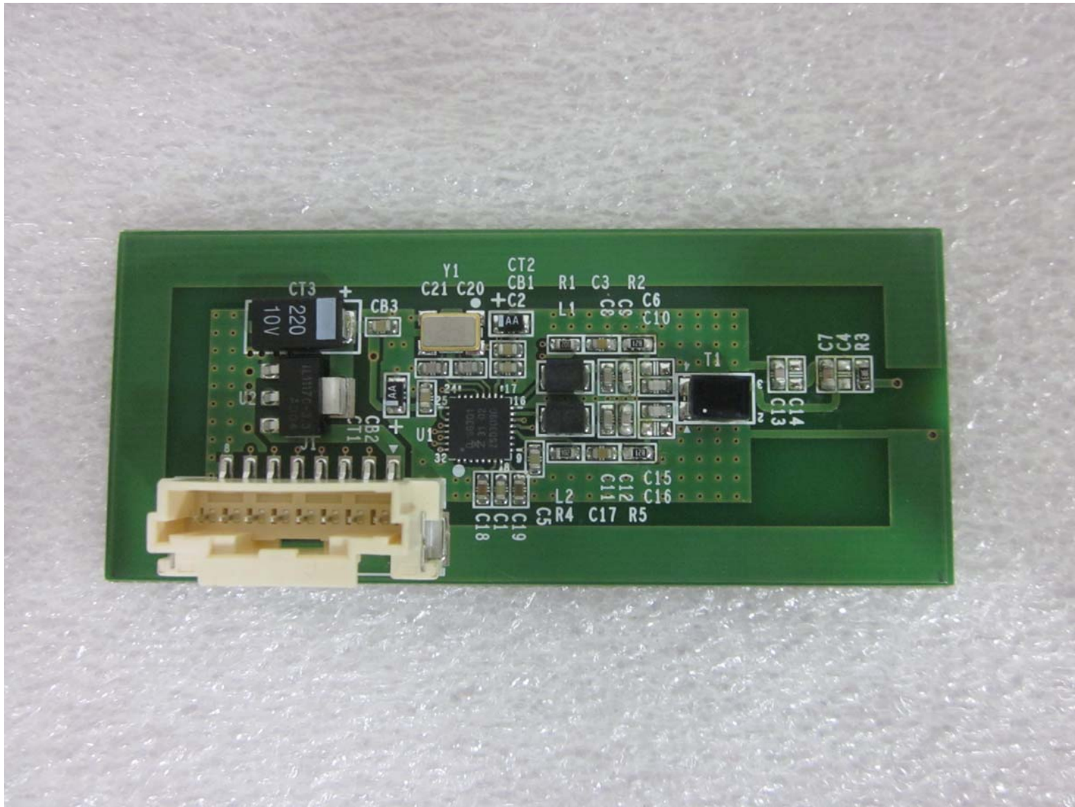
SMT-500P_RFID Board Rear
