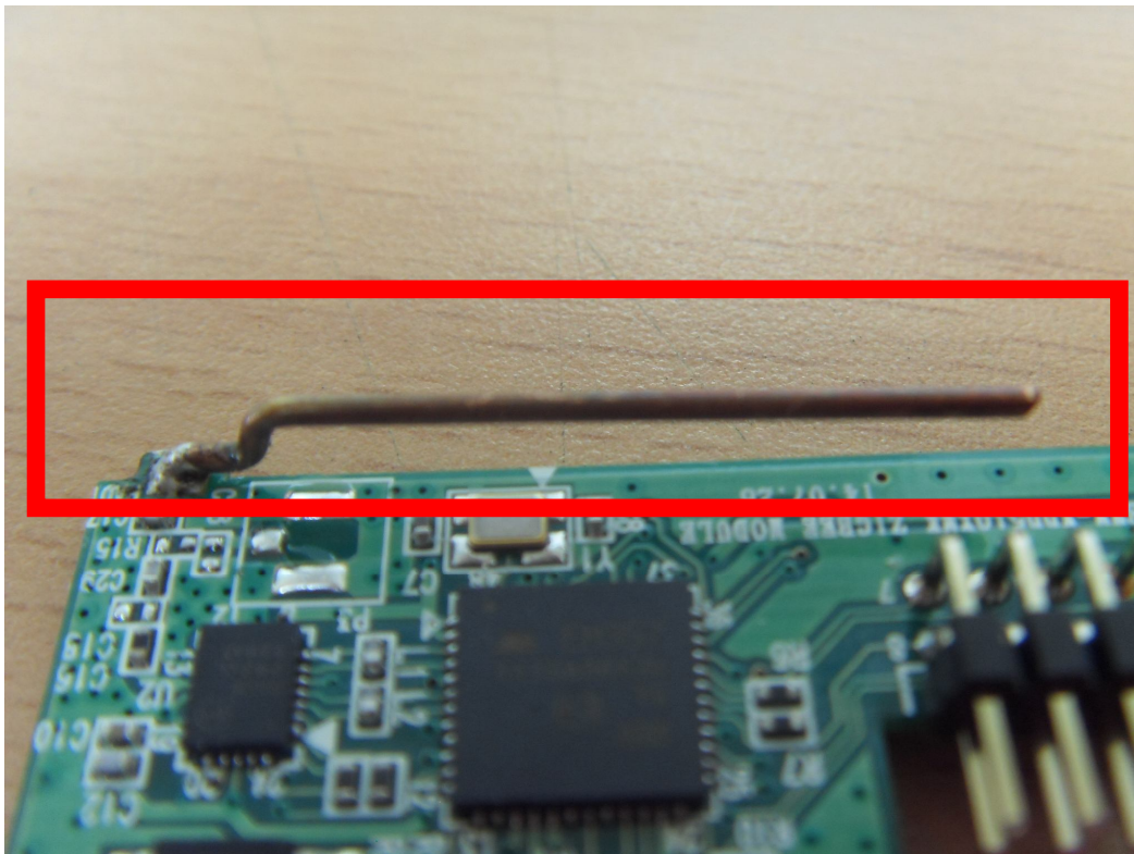
Zigbee Antenna
