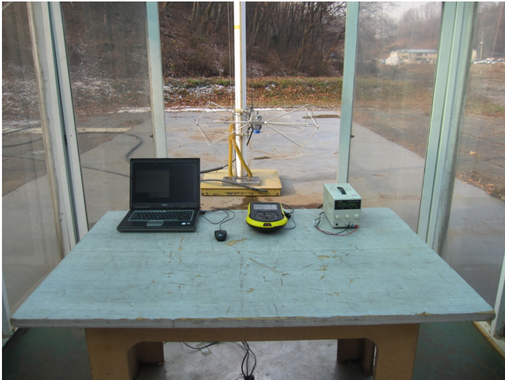
Radiated RF measurement (Below 1 GHz)
