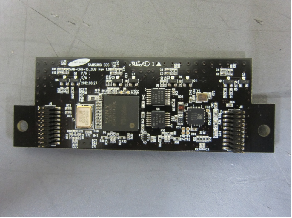
Sub Board 1_Front
