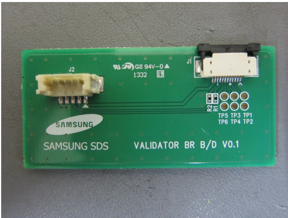
Sub Board 2_Front
