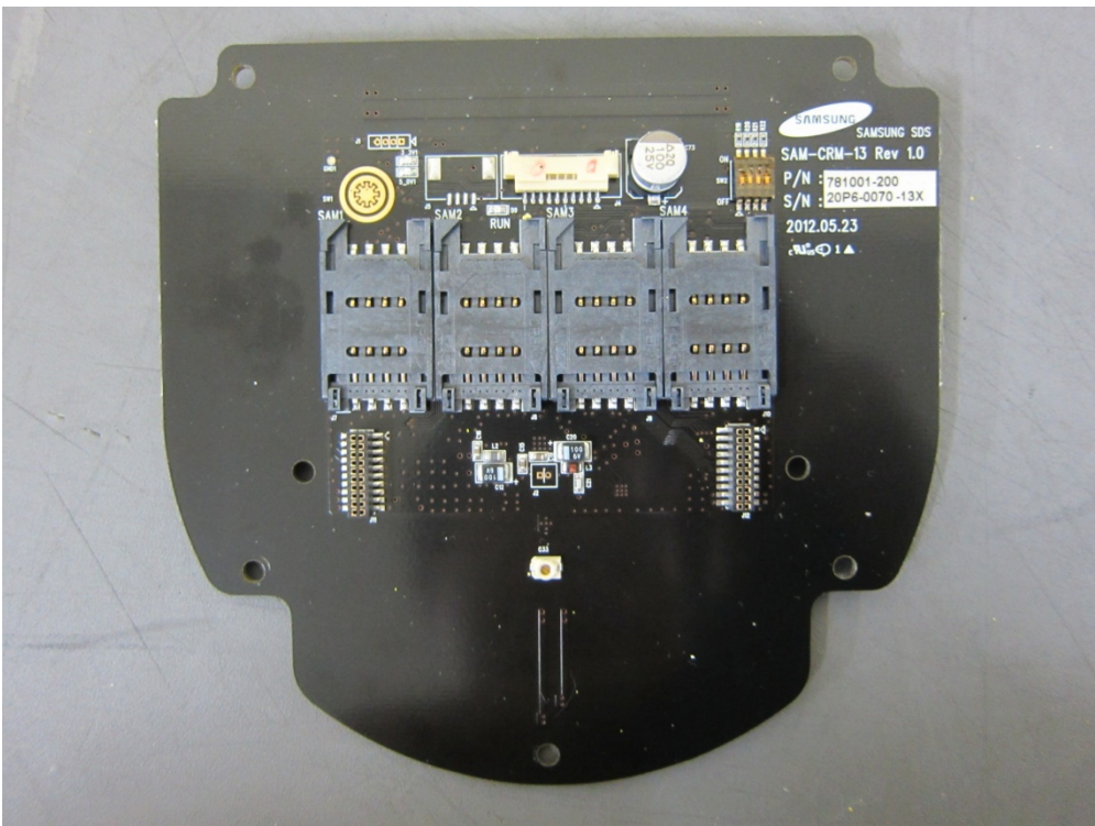
RFID Board Rear
