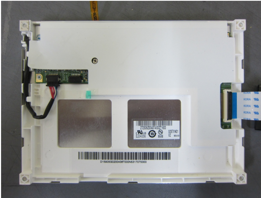
LCD Board Rear
