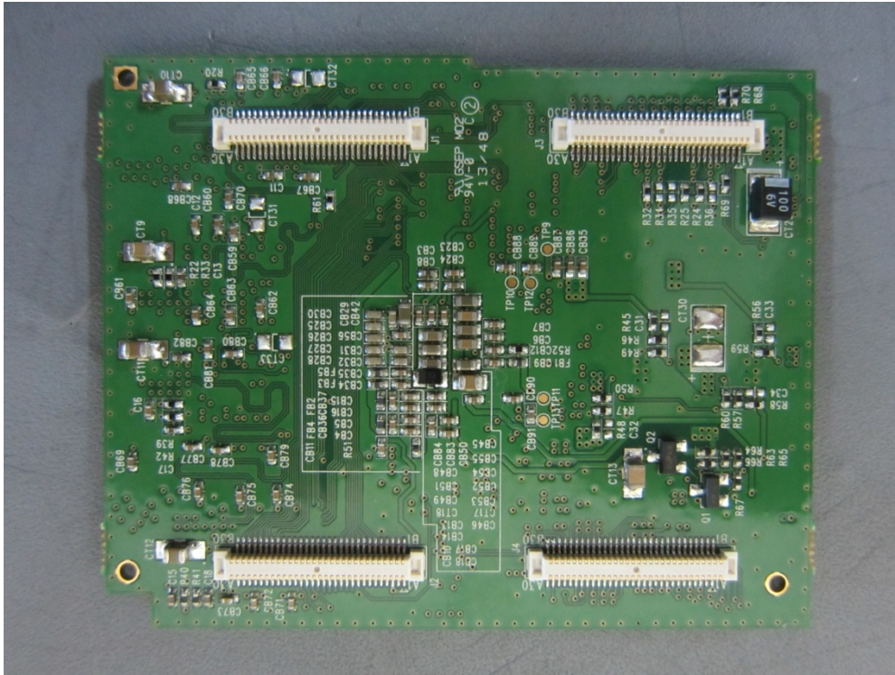
Control Board Rear
