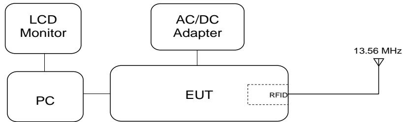
[System Block Diagram of Test Configuration]
