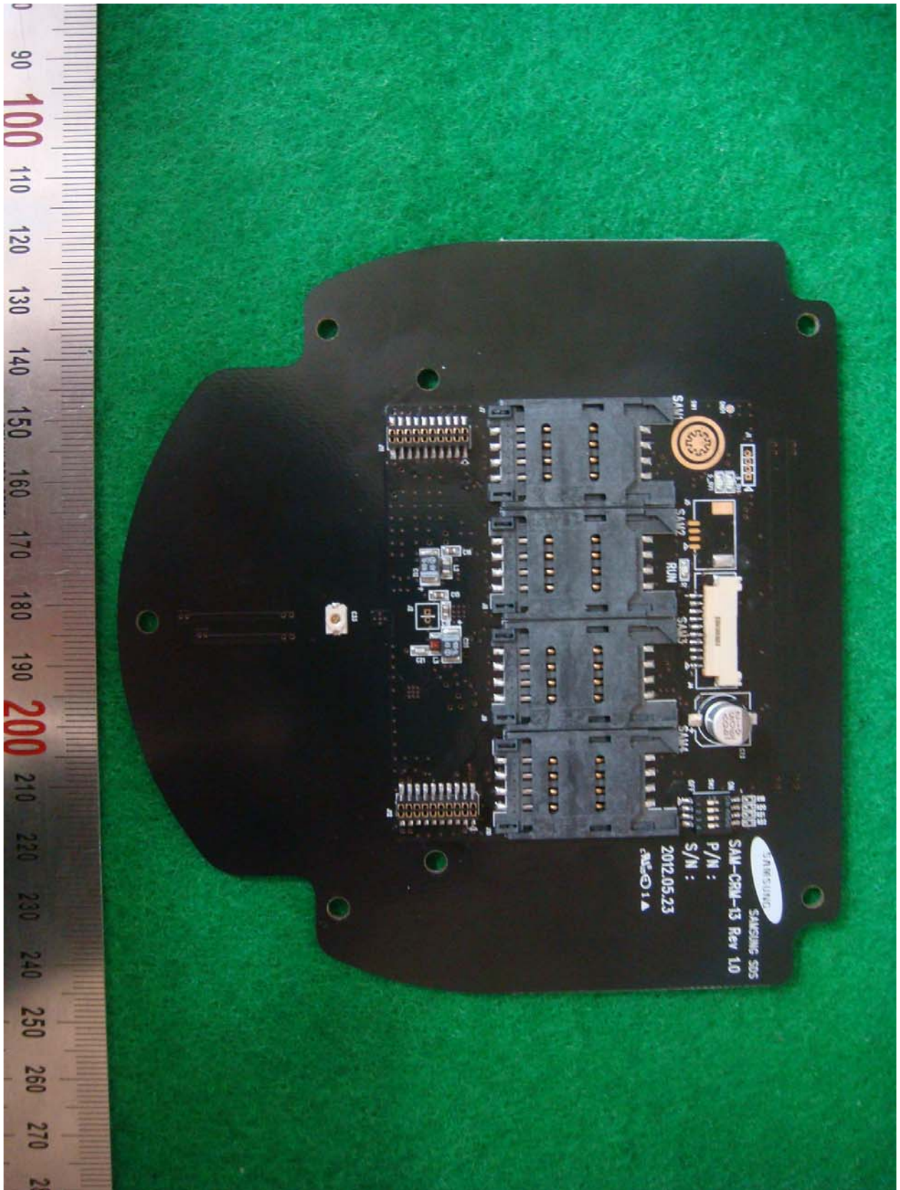
<Photograph 4: Main board (Sub board removed) - Rear view>
