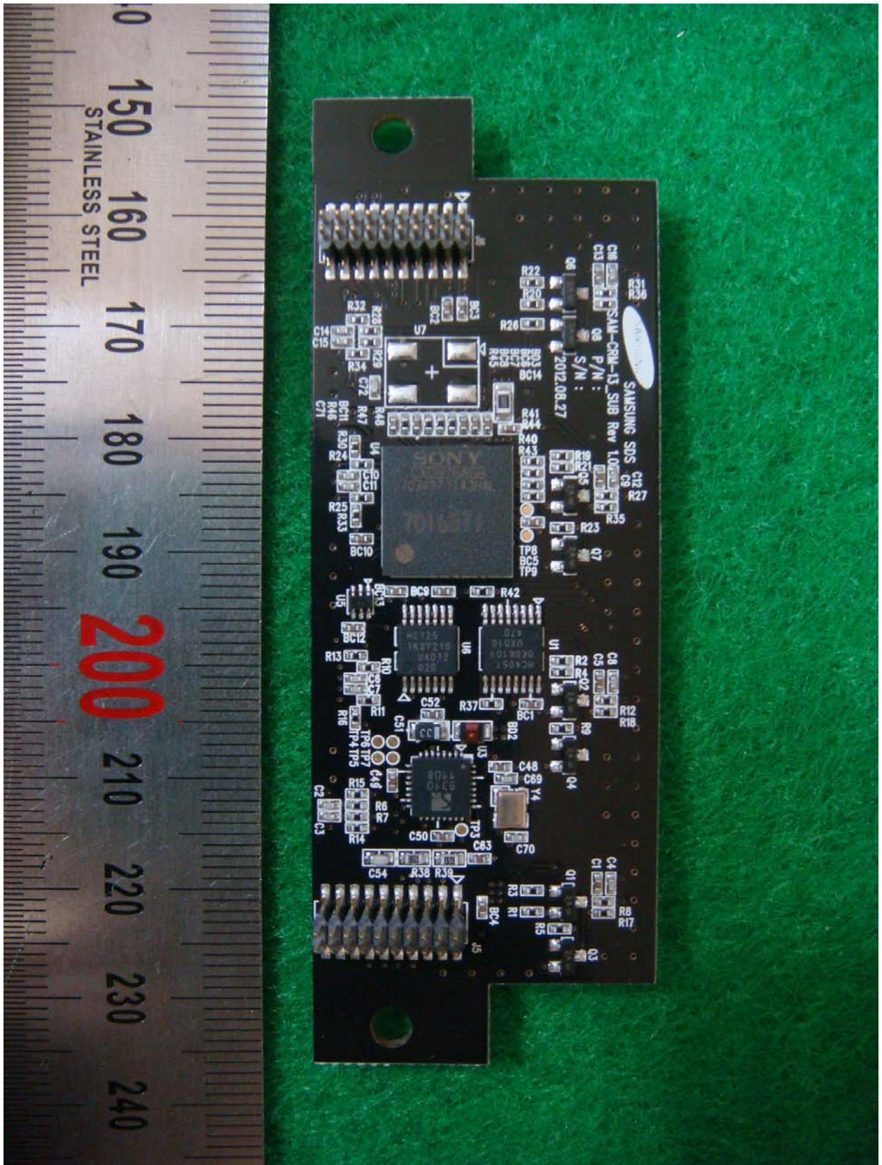
<Photograph 5: Sub board - Front view>
