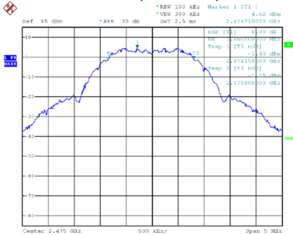
F5 (2 475 MHz)
