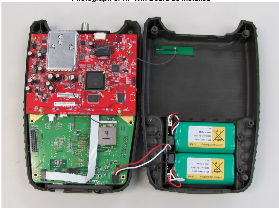
Photograph of RF Wifi Board as Installed
