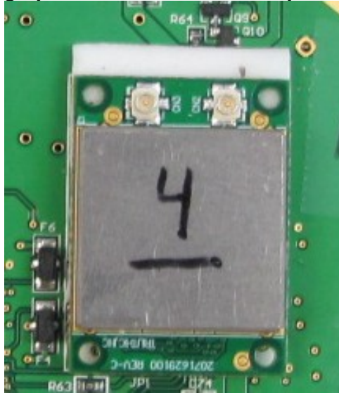
Photograph of RF Wifi Board: Component Side – Shield removed
