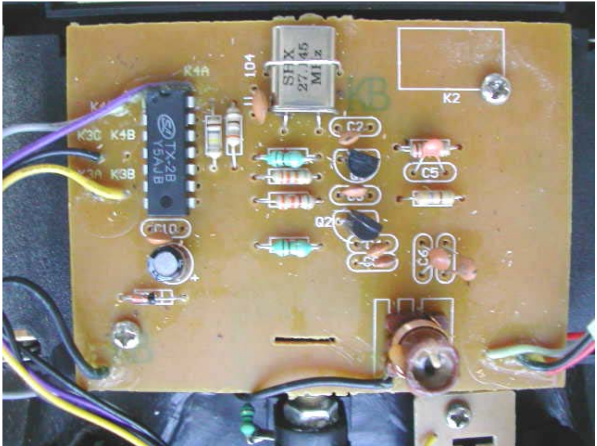
(Inner circuit board 1)
