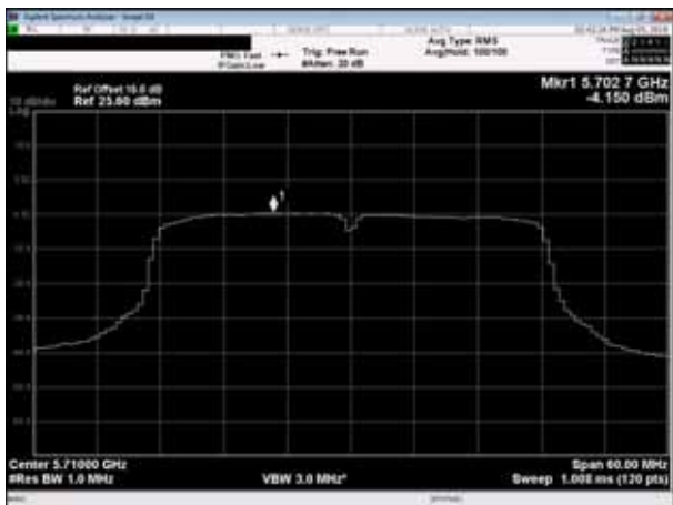
Channel 142 (5710MHz)
