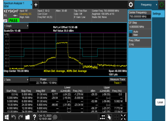
Emission Mask_Band14_5MHz_QPSK_RB25_0_CH23330
