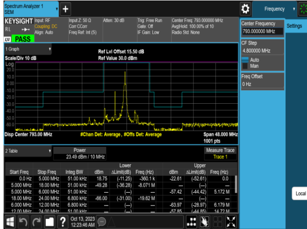
Emission Mask_Band14_5MHz_QPSK_RB1_24_CH23330
