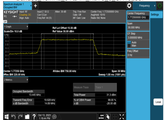
Band66_15MHz_64QAM_RB75_0_CH132597
