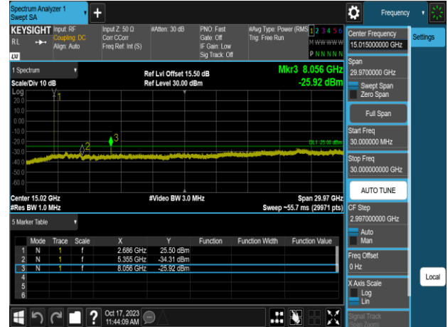
Band41_5MHz_QPSK_RB1_0_CH41565
