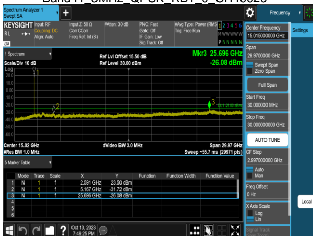
Band41_5MHz_QPSK_RB1_0_CH40620
