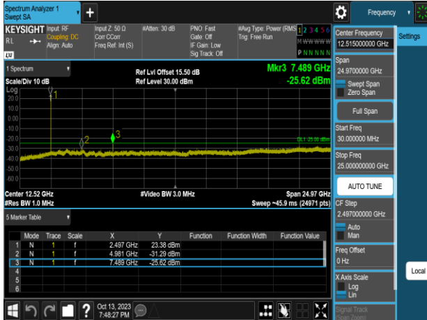
Band41_5MHz_QPSK_RB1_0_CH39715
