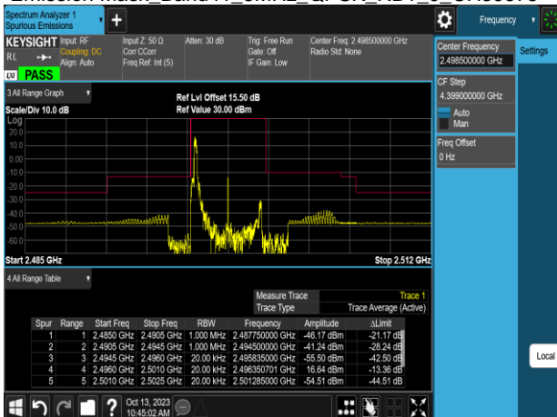
Emission Mask_Band41_5MHz_QPSK_RB1_0_CH39675
