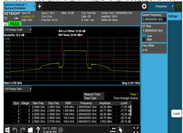
Emission Mask_Band7_10MHz_QPSK_RB50_0_CH21400
