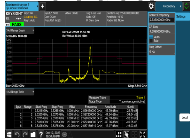
Emission Mask_Band7_5MHz_QPSK_RB1_24_CH21425
