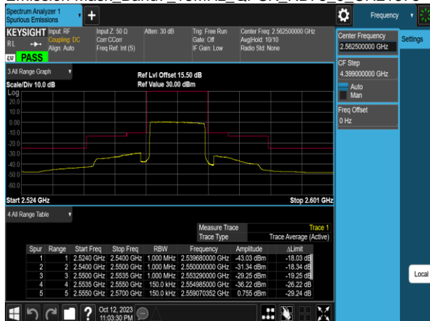
Emission Mask_Band7_15MHz_QPSK_RB75_0_CH21375
