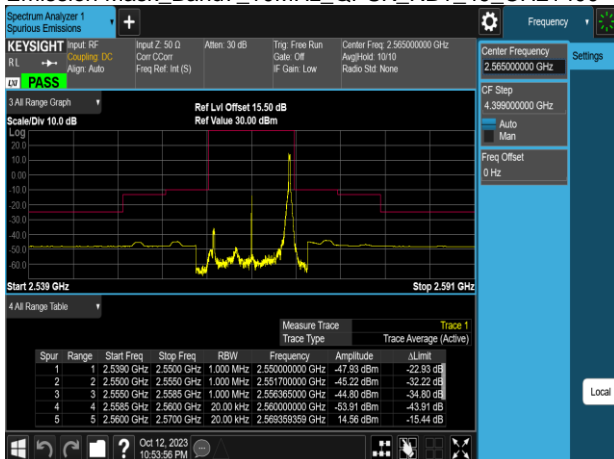
Emission Mask_Band7_10MHz_QPSK_RB1_49_CH21400
