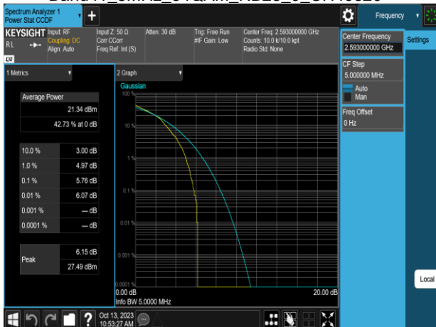
Band41_5MHz_64QAM_RB25_0_CH40620
