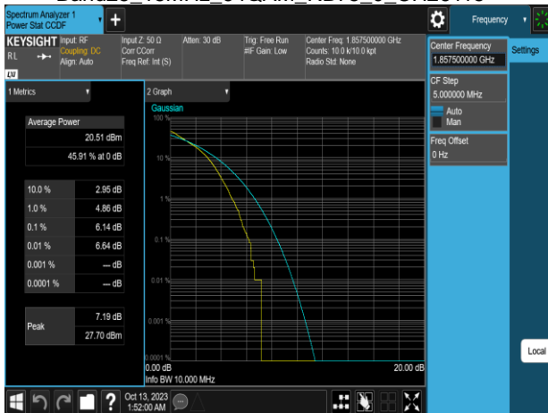
Band25_15MHz_64QAM_RB75_0_CH26115
