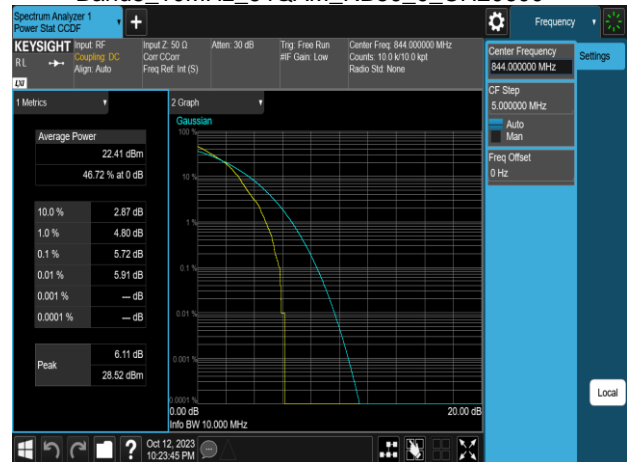
Band5_10MHz_64QAM_RB50_0_CH20600
