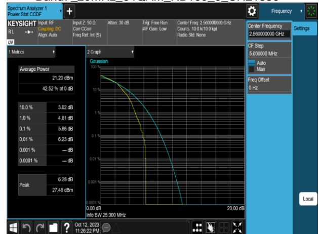
Band7_20MHz_64QAM_RB100_0_CH21350
