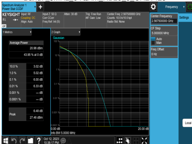
Band7_5MHz_64QAM_RB25_0_CH21425
