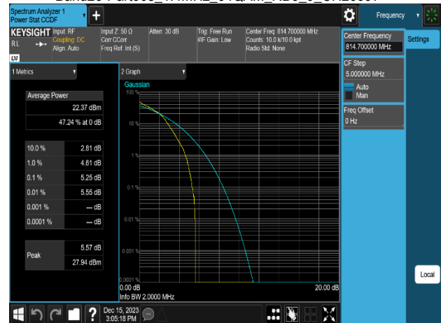
Band26-Part90s_1.4MHz_64QAM_RB6_0_CH26697
