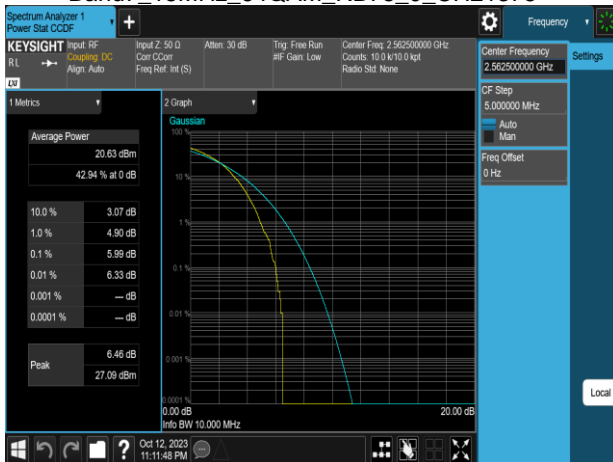
Band7_15MHz_64QAM_RB75_0_CH21375
