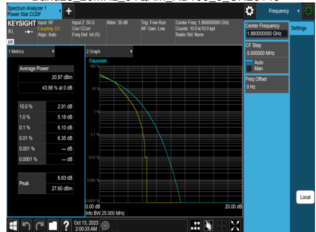
Band25_20MHz_64QAM_RB100_0_CH26140
