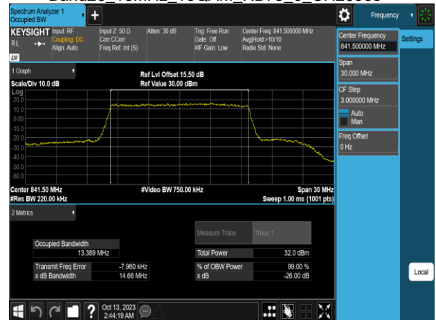
Band26_15MHz_16QAM_RB75_0_CH26965
