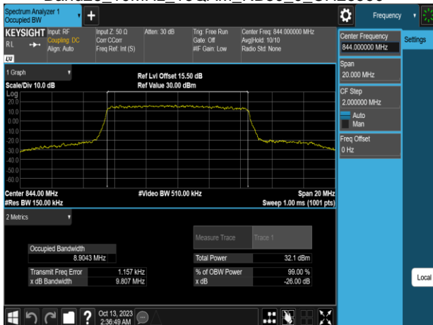
Band26_10MHz_16QAM_RB50_0_CH26990
