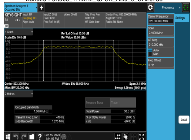
Band26-Part90s_1.4MHz_QPSK_RB6_0_CH26783
