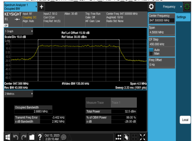
Band26_3MHz_QPSK_RB15_0_CH27025
