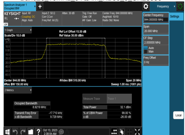
Band26_10MHz_64QAM_RB50_0_CH26990
