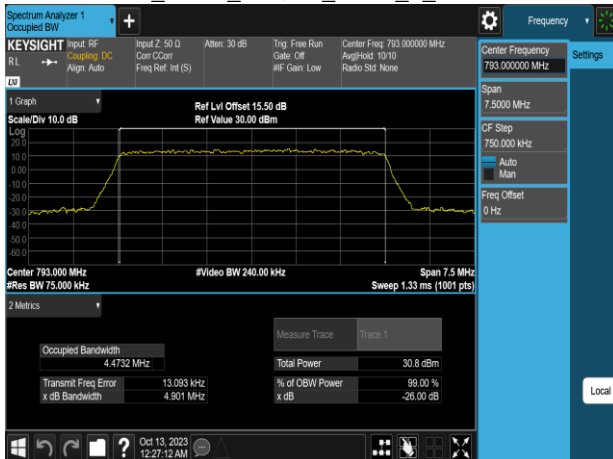
Band14_5MHz_64QAM_RB25_0_CH23355
