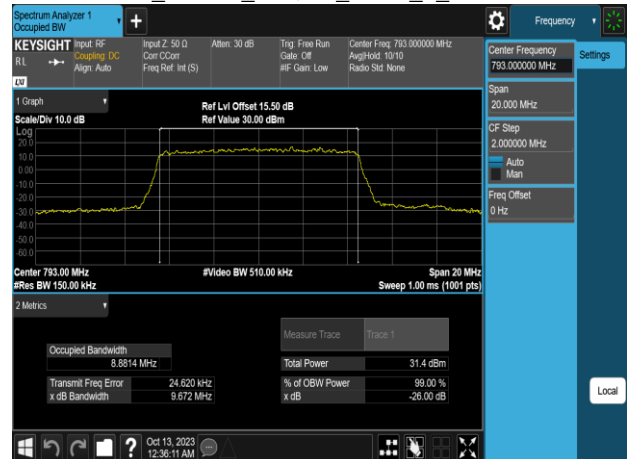
Band14_10MHz_64QAM_RB50_0_CH23330
