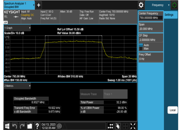
Band14_10MHz_16QAM_RB50_0_CH23330
