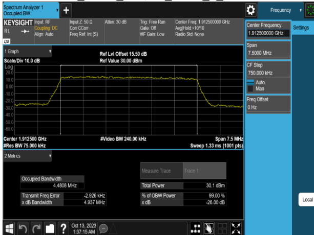
Band25_5MHz_64QAM_RB25_0_CH26665
