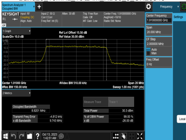
Band25_10MHz_16QAM_RB50_0_CH26640
