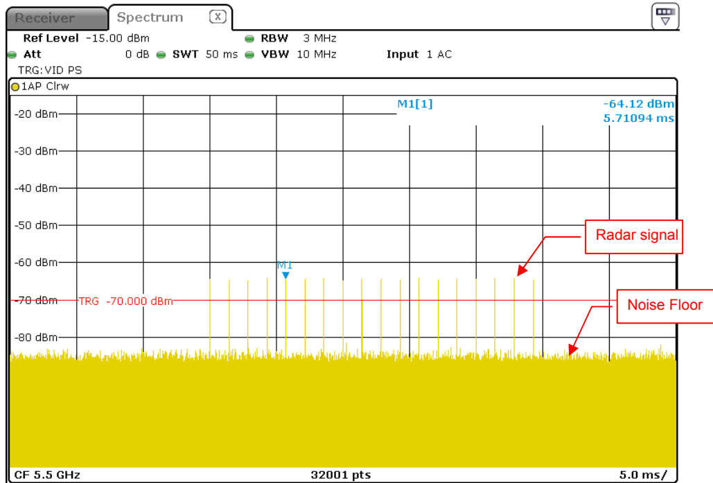
Radar Signal 0
