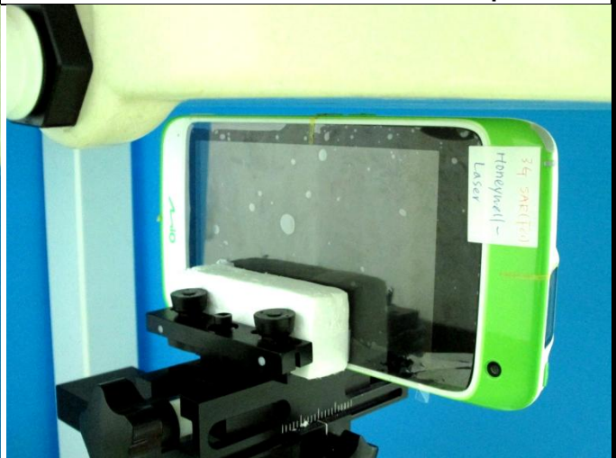
Left Side of EUT with 5 mm Gap
