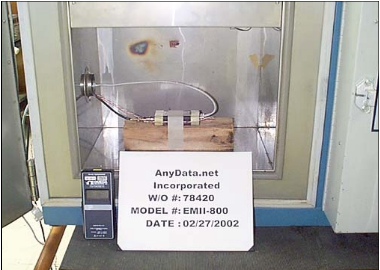
Temperature Testing Setup
