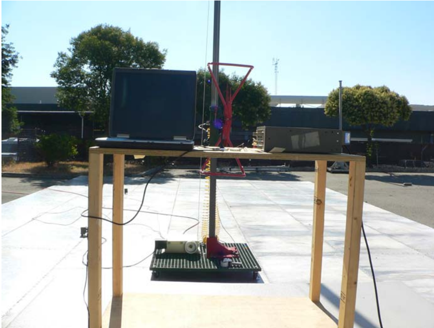
Transmitter Radiated Emission - Front View
