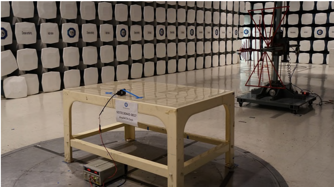
Radiated Emissions Below 1GHz Rear
