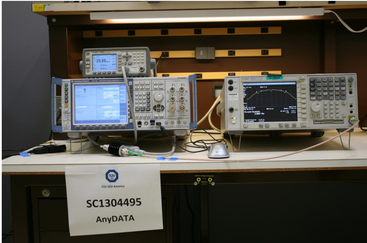
Conducted Port Test Setup (Unlicensed)
