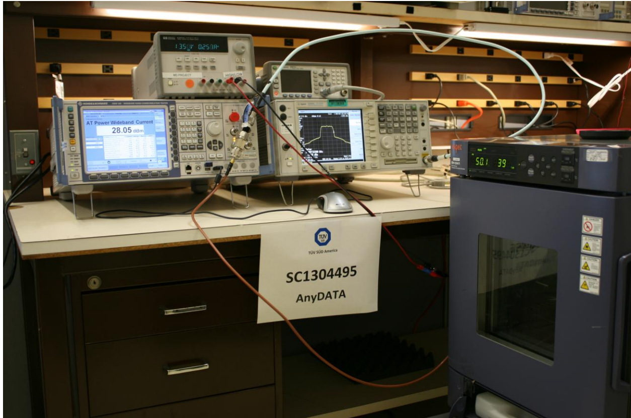
Conducted Port Test Setup (Licensed)
