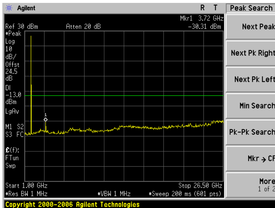
Plot 2d: 1 GHz –26.5 GHz
