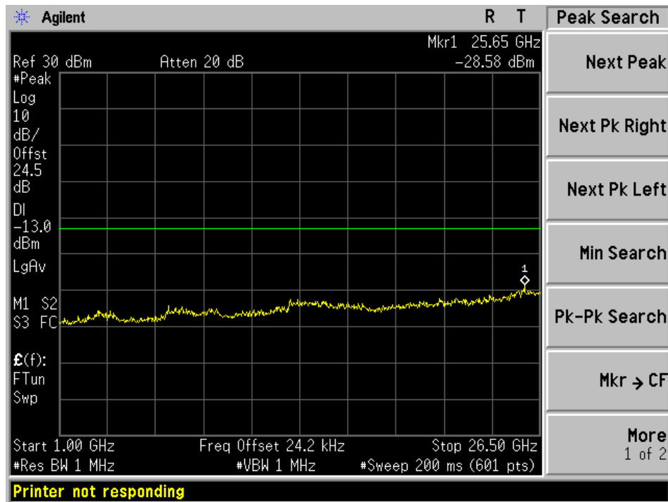
Plot 2c: 1 GHz – 26.5 GHz
