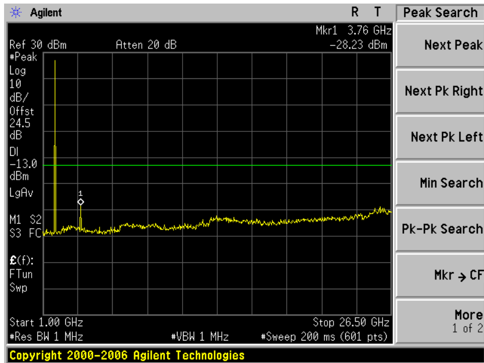
Plot 2e: 1 GHz –26.5 GHz
