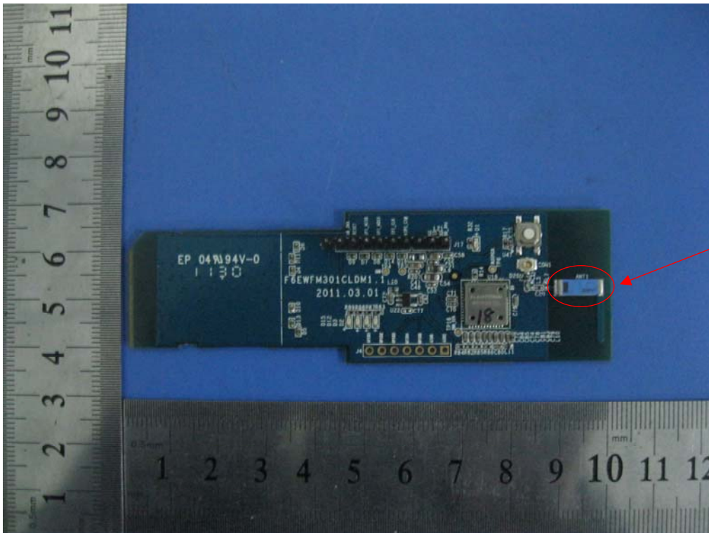
External Antenna
