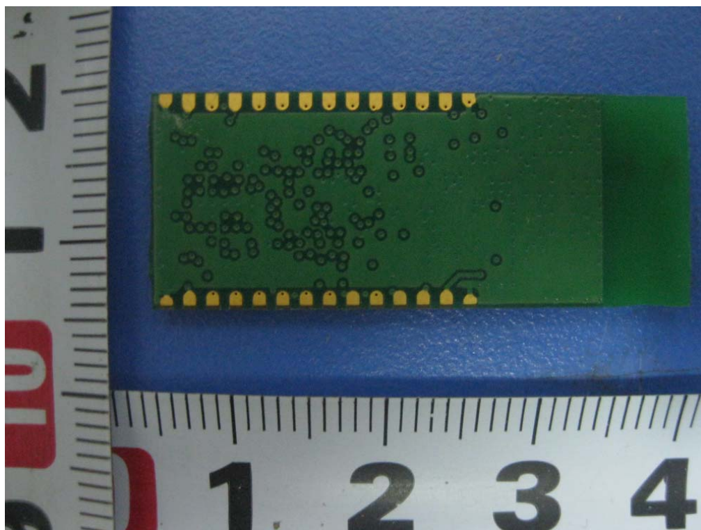
BT Antenna - Front View
