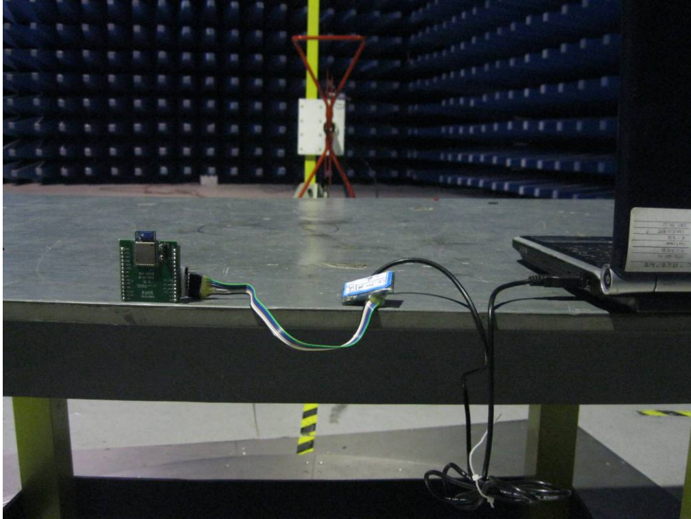
Radiated Emissions Test Setup Below 1GHz - Rear Closer View
