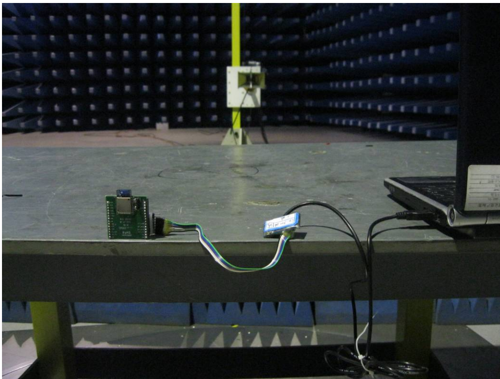
Radiated Emissions Test Setup Above 1GHz – Rear Closer View
