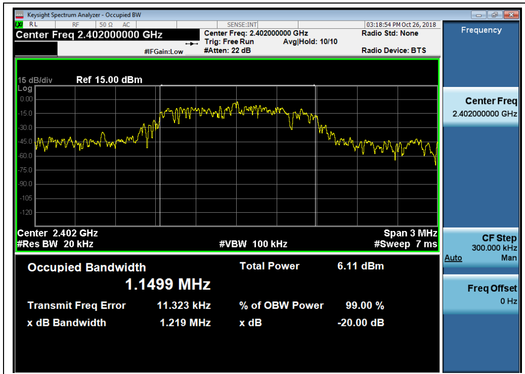
(8-DPSK, Channel 0, 2402MHz)
