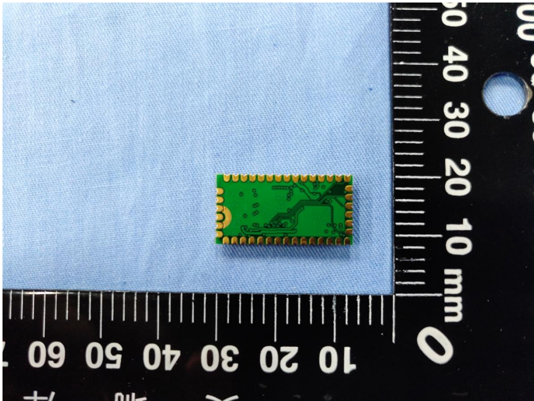
2.bottom view
