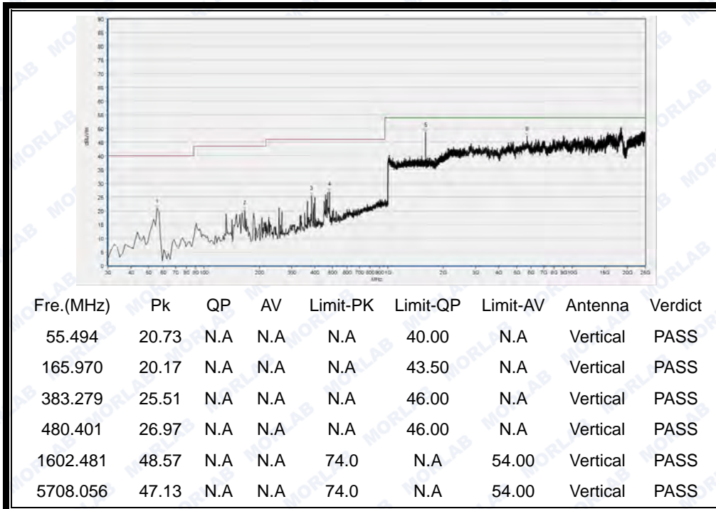
(30MHz to 25GHz, Antenna Vertical @ GFSK, channel 0)
