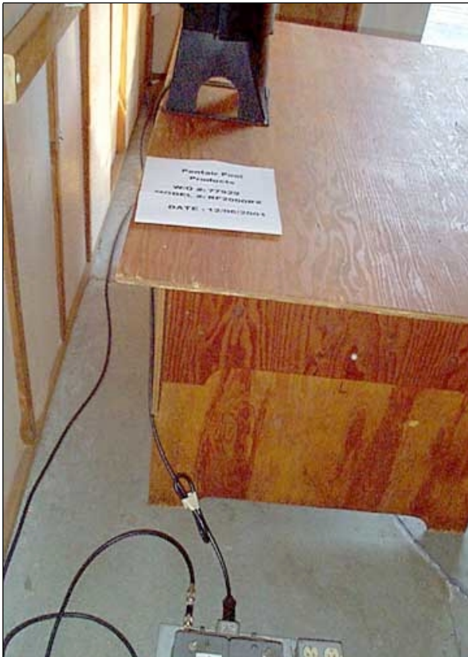
Mains Conducted Emissions - Side View of Receiver
