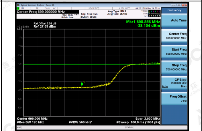
LCH_16QAM_50RB#0
