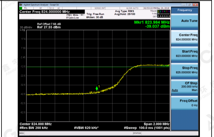
LCH_16QAM_50RB#0
